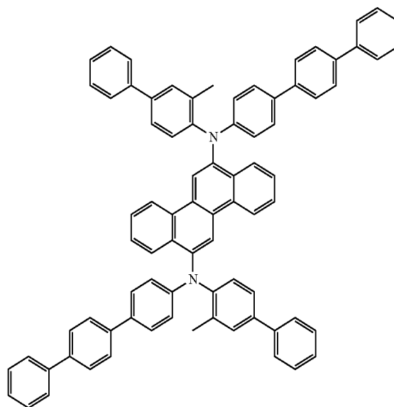
C 80 H 68 N 2 Exact Mass: 1046.46 Mol. Wt.: 1047.33 C, 91.74; H, 5.58; N, 2.67
