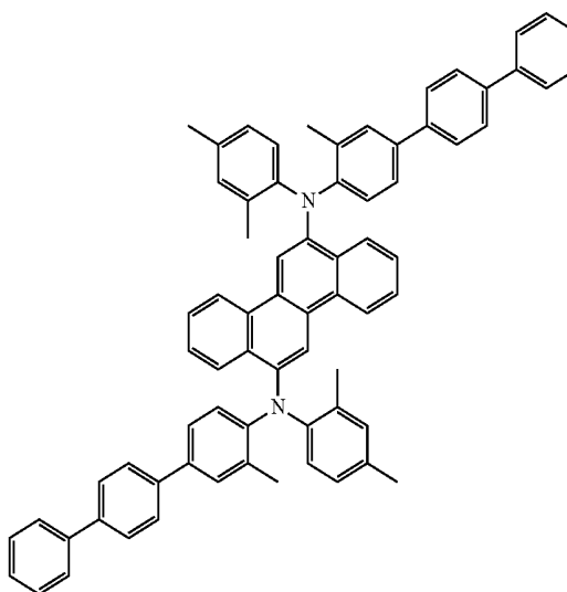
C 72 H 58 N 2 Exact Mass: 950.46 Mol. Wt.: 951.24 C, 90.91; H, 6.15; N, 2.94
